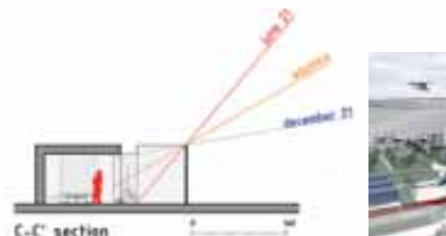
C-C' section
