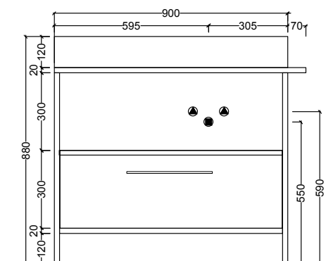
90 BACINO DX + CASSETTO 90 RIGHT WASHBASIN + DRAWER
