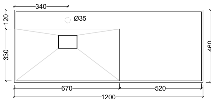
120 BACINO DX / SX 120 LEFT / RIGHT WASHBASIN
