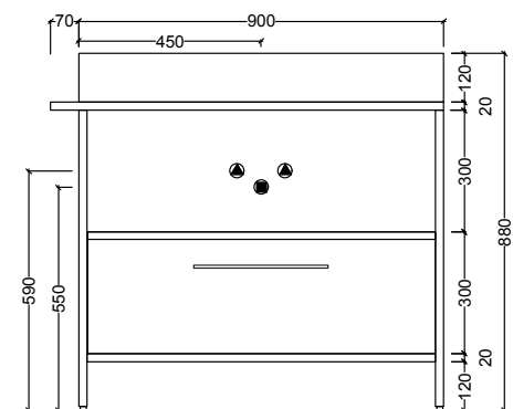
90 BACINO UNICO + CASSETTO 90 SINGLE WASHBASIN + DRAWER
