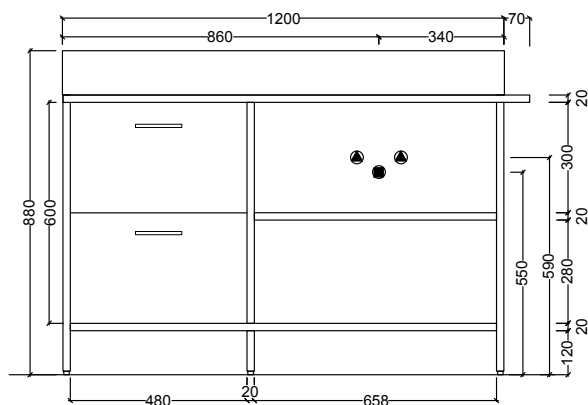
120 BACINO DX + CASSETTI 120 RIGHT WASHBASIN + DRAWERS
